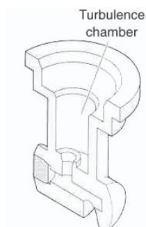
Pre-orifice flood nozzle with turbulence chamber
