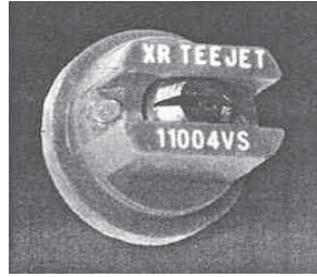
Nozzle that operates at low pressure (extended range nozzle)
